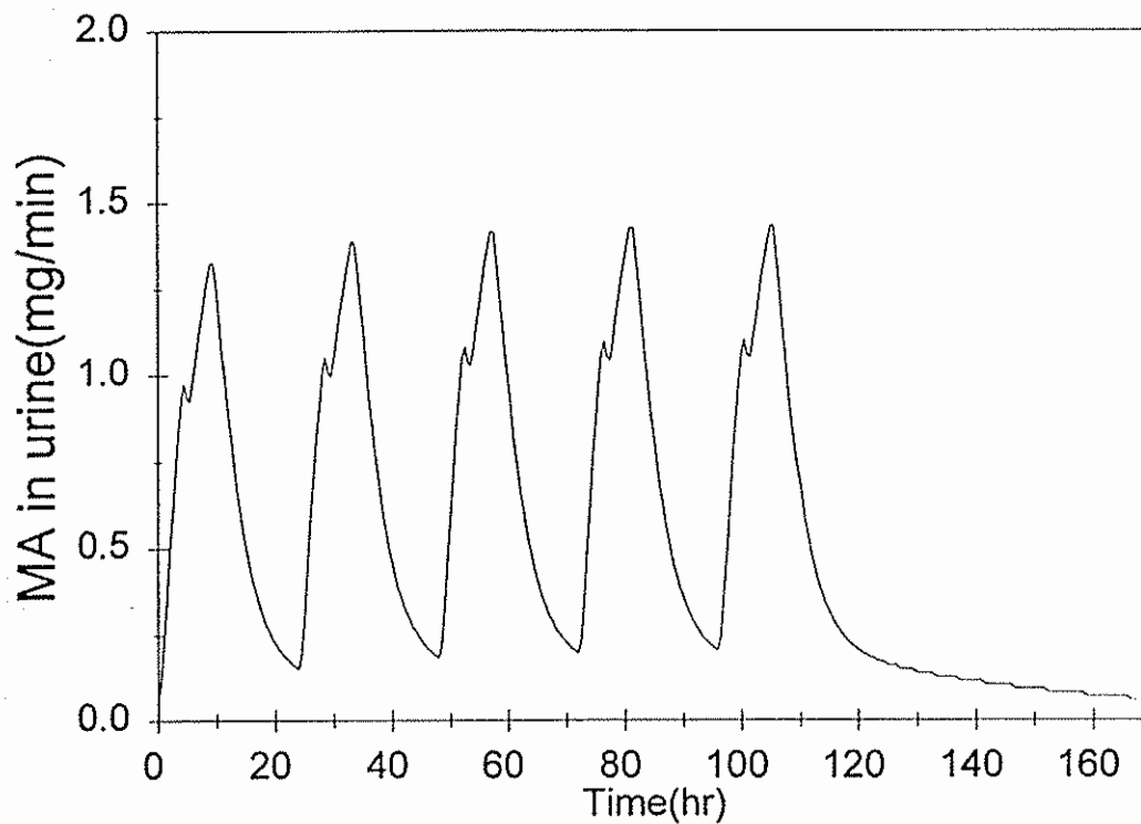
Fig. 10. Simulation of urinary mandelic acid concentration during an occupational exposure to 50 ppm styrene: 8 hours/day with 1 hour break, 5 days/week
