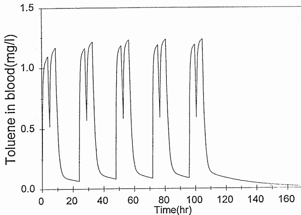
Fig. 6. Simulation of venous blood toluene concentration during an occupational exposure to 50 ppm toluene: 8 hours/day with 1 hour break, 5 days/week
