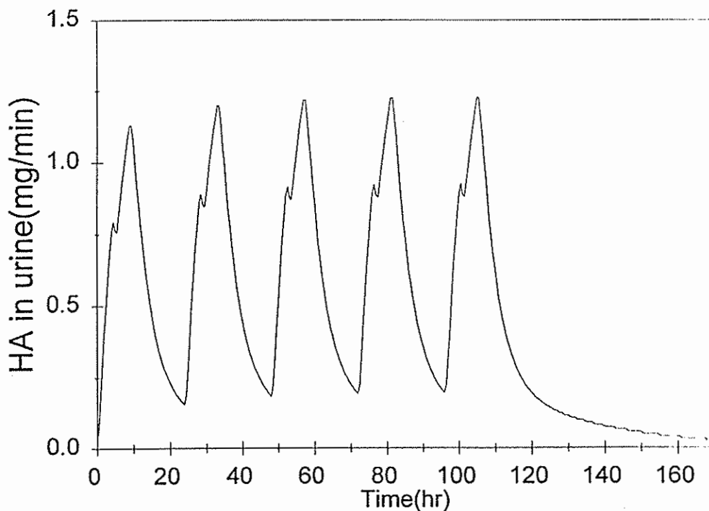
Fig. 7. Simulation of urinary hippuric acid concentration during an occupational exposure to 50 ppm toluene: 8 hours/day with 1 hour break, 5 days/week
