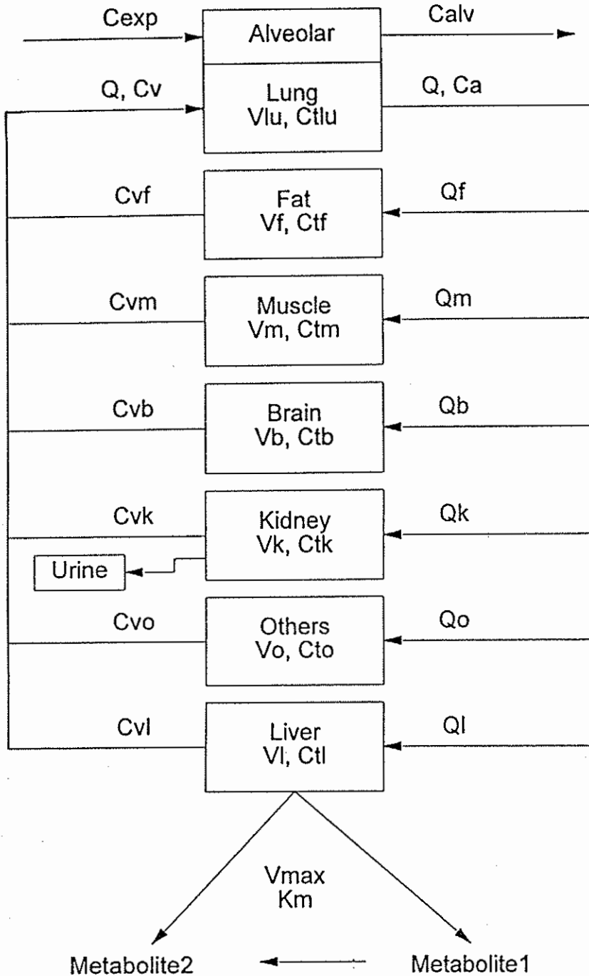
Fig. 1. Structure of PB-PK model(Ca, arterial concentration; Cv, venous concentration; Q, blood flow; Cexp, exposure concentration; Calv, alveolar concentration; V, tissue volume; Ct, concentration in tissue)
